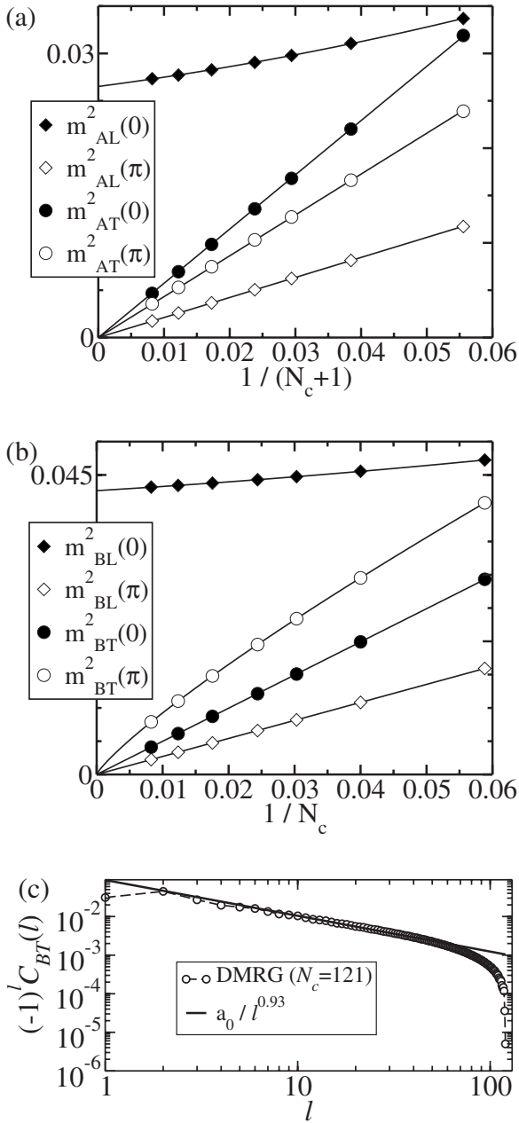
FIG. 3. DMRG results for the square of the longitudinal ( L ) and transverse ( T ) order parameters at the spin sector S^z=S_g and J=0.395 for (a) A and (b) B ( B_1 or B_2 ) spins (full lines are polynomial fittings). (c) DMRG results for the transverse staggered correlation function C_{BT\pi}(l) .
