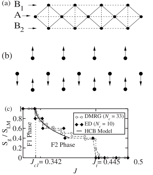
FIG. 1. (a) Illustration of the A and B sublattices (circles) and AF spin couplings, which favor (full lines) and destabilize (dashed lines) the LM ferrimagnetic GS: J_1(\equiv 1) and J , respectively. (b) Illustration of the LM ferrimagnetic GS. (c) Results (see text) for S_g/S_{LM} ; dashed and dotted lines are guides to the eye.
