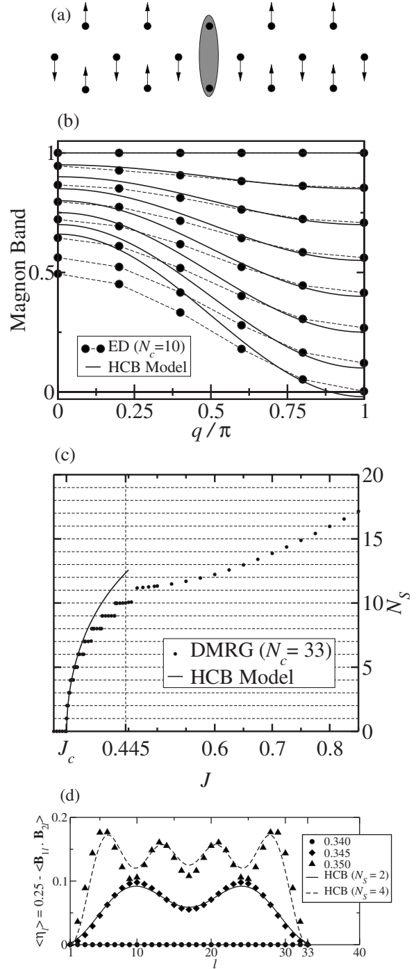
FIG. 4. (a) Illustration of the relevant magnon excitation for J=0 : ellipse indicates a local singlet state. (b) Magnon band for J=0.00, 0.05, 0.10, 0.15, 0.20, 0.25, 0.30, and 0.34 , from top to bottom. (c) N_S as a function of J . Full lines are the HCB model predictions in the TG limit and dashed lines are guides to the eye.
