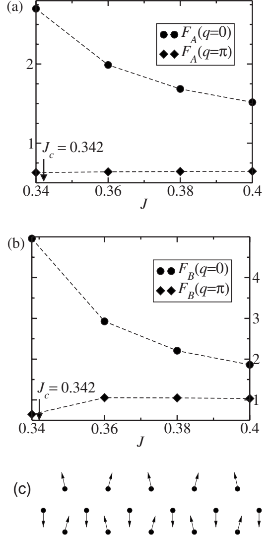
FIG. 2. DMRG results for the magnetic structure factor, F_X(q) , at q=0 and q=\pi for (a) X=A and (b) X=B ( B_1 or B_2 ) spins in a chain with N_c=33 ; dashed lines are guides to the eye. (c) Illustration of the F2 phase.
