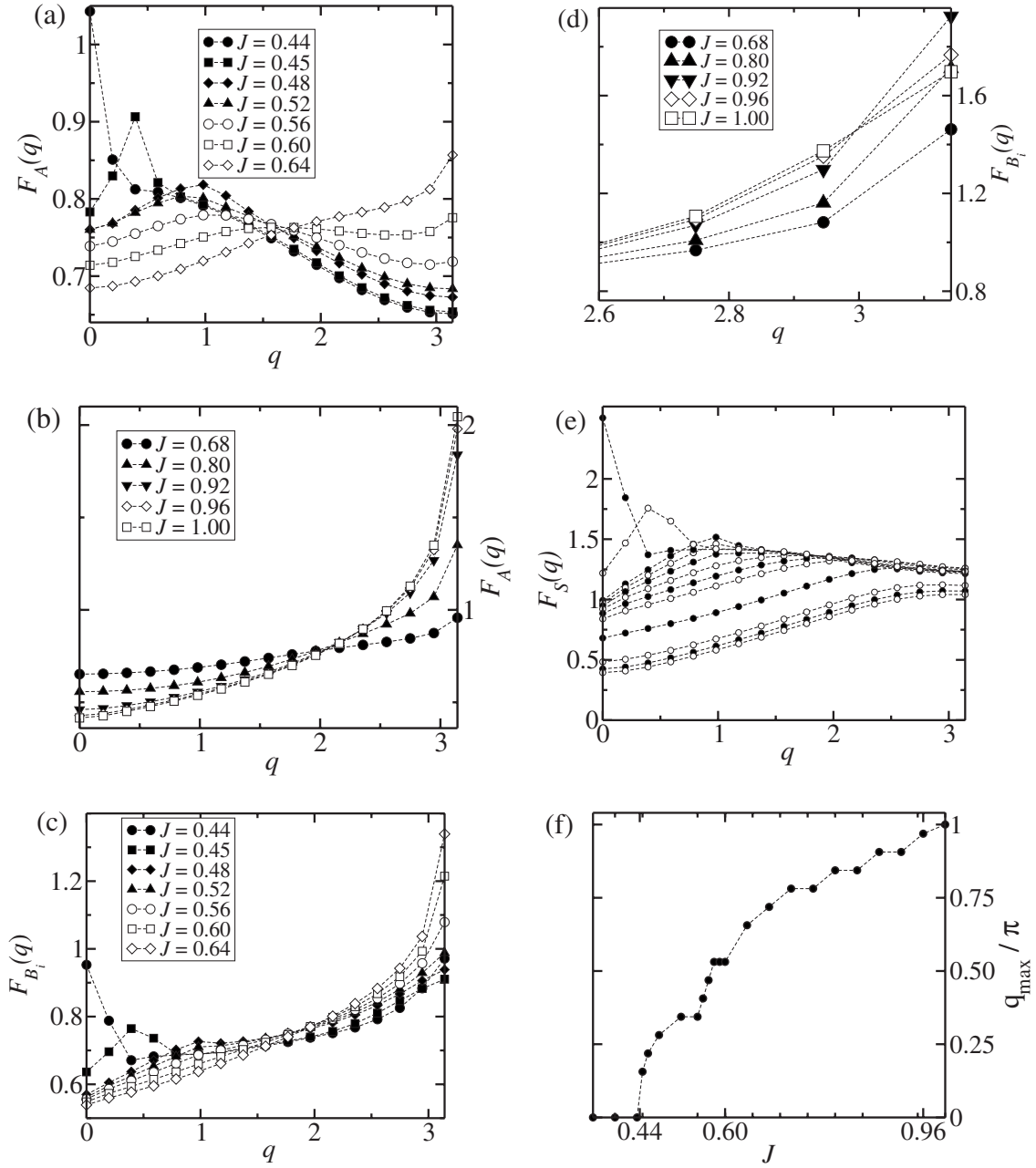
FIG. 6. Magnetic structure factor F_X(q) for the A spins [(a) and (b)], N_c=32 , and for the B_i spins [(c) and (d) with i=1 or 2 ], N_c=33 , for the indicated values of J . (e) Magnetic structure factor for the composition S_l = \mathbf{B}_{1l} + \mathbf{B}_{2l} and J=0.44, 0.45, 0.48, 0.52, 0.56, 0.60, 0.64, 0.68, 0.80, 0.92, 0.96 , and 1.00 , from top to bottom at q=0 . (f) The value of the wave vector, for which the peak at the magnetic structure factor exhibited in (e), is observed. Dashed lines are guides to the eye.
