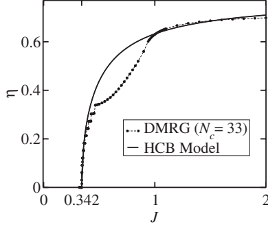
FIG. 8. Density of singlets as function of J .
