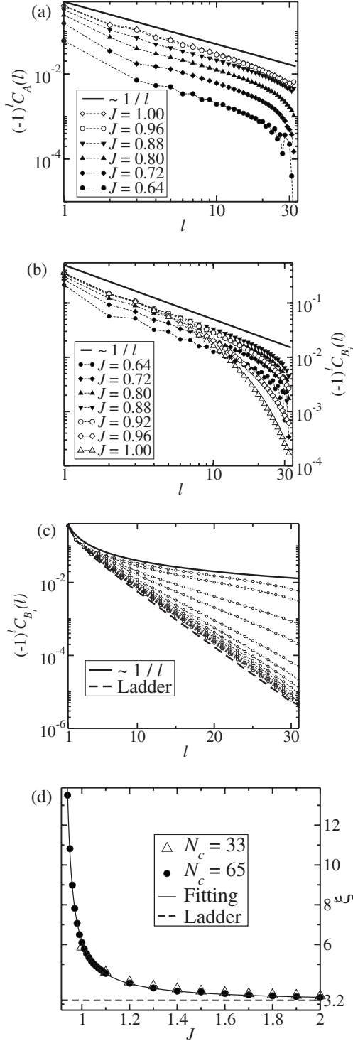
FIG. 7. Staggered correlation functions between (a) A spins, N_c=32 , and (b) B_i (with i=1 or 2 ) spins, N_c=33 , for the indicated values of J . In (a) and (b) solid lines indicate the asymptotic behavior for a single chain. (c) Staggered correlation functions between B_i (with i=1 or 2 ) spins for J=0.88, 0.92, 0.96, 1.0, 1.1, 1.2, 1.3, 1.4, 1.5, 1.6, 1.7, 1.8, 1.9 , and 2.0 , circles-dash from top to bottom and N_c=33 . For comparison we plot the behavior for a single chain (solid line) and for a two-leg ladder with 32 rungs. (d) Correlation length \xi as a function of J : solid line indicates the fitting of the data for N_c=65 to Eq. (33) with g given by Eq. (40); dashed line indicates the value of \xi ( \approx 3.2 ) for a two-leg ladder.
