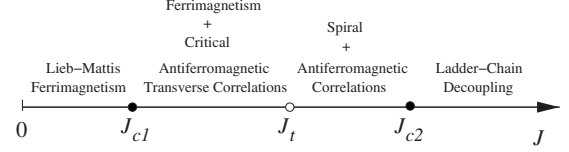
FIG. 9. Schematic representation of the phase diagram.
