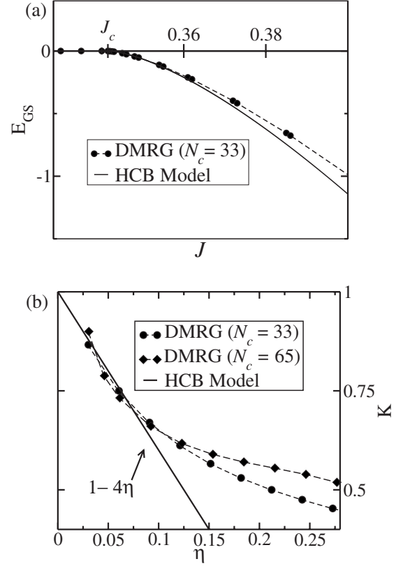
FIG. 5. (a) Ground-state energy, E_{GS} , relative to the energy of the LM state. (b) Luttinger liquid exponent, K , as function of \eta . Full lines are the HCB model predictions in the TG limit and dashed lines are guides to the eye.
